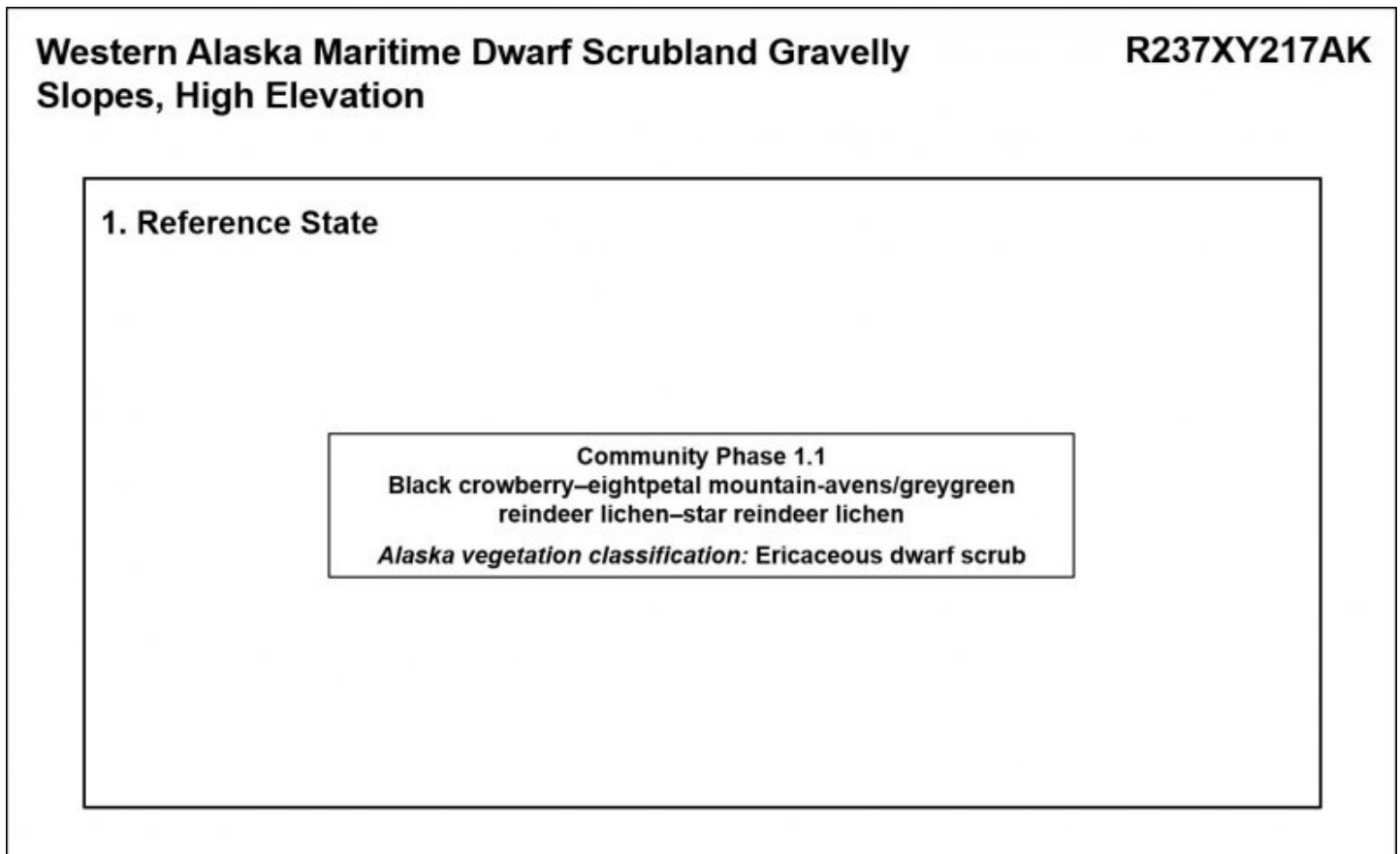
Figure 4. State-and-transition model.
