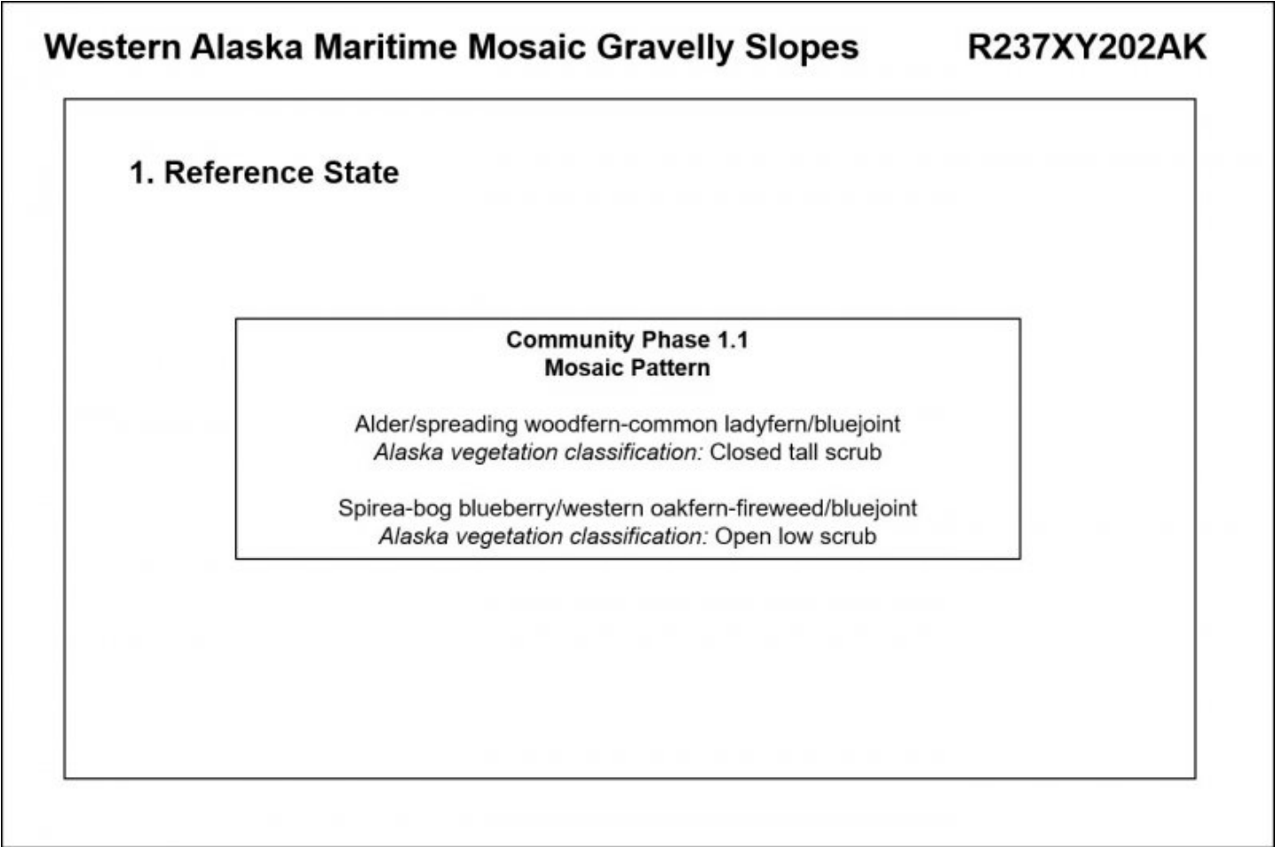
Figure 5. State-and-transition model.
