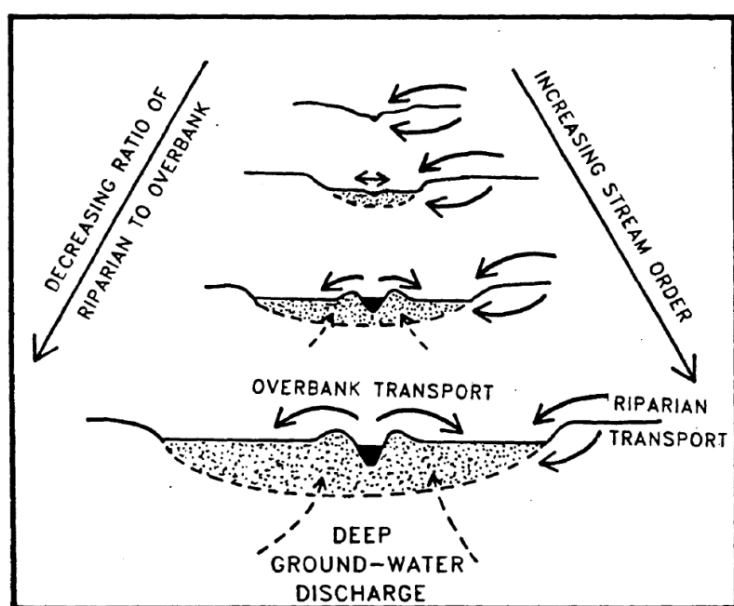
Figure 13. An illustration of the effect of stream order on 1) the severity of overbank flooding, and 2) the ratio of soil water derived from overbank flooding to the amount derived from overland water and groundwater moving towards the stream. From Brinson (1993).
