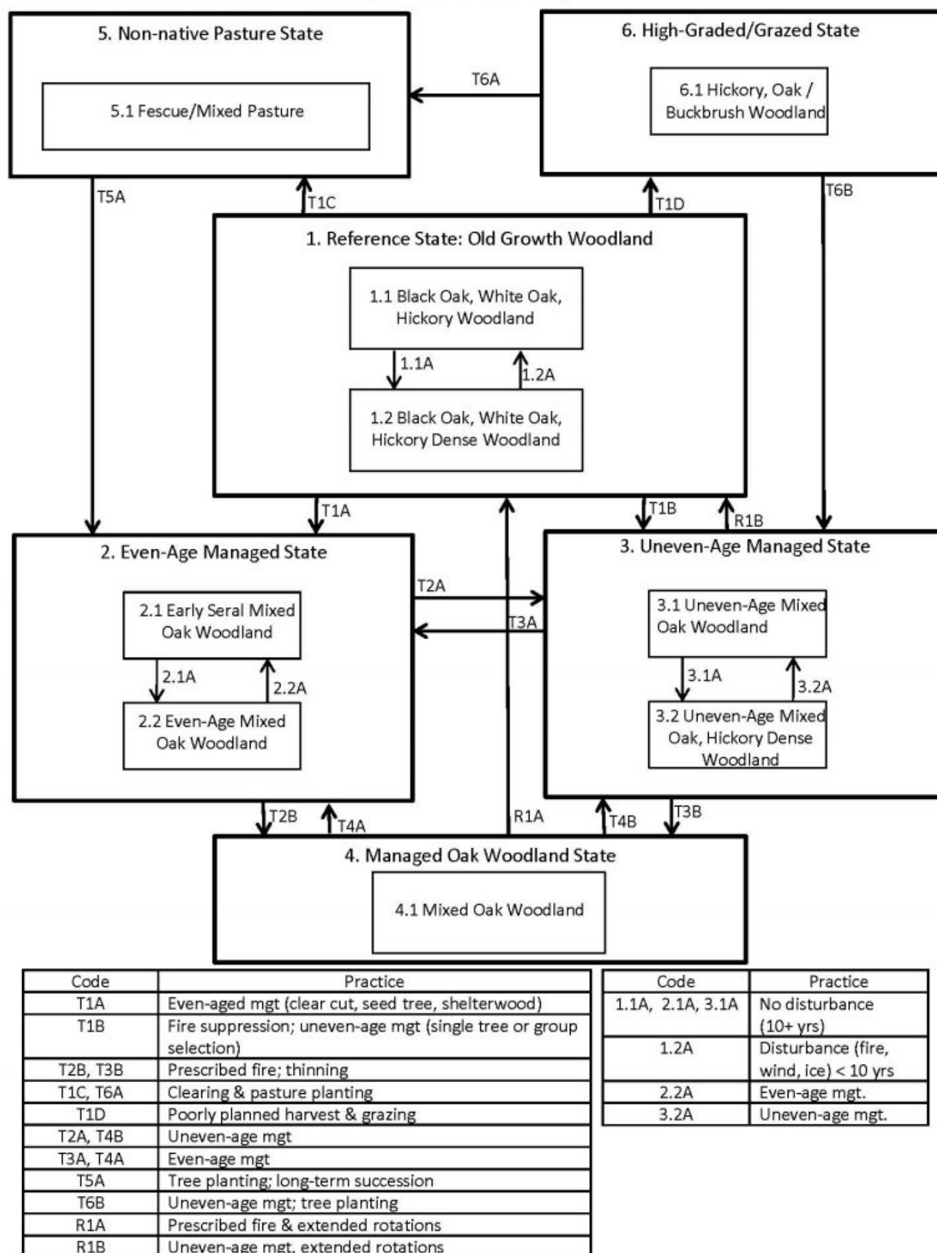
Figure 8. Alflic Chert Exposed Backslope Woodlands
