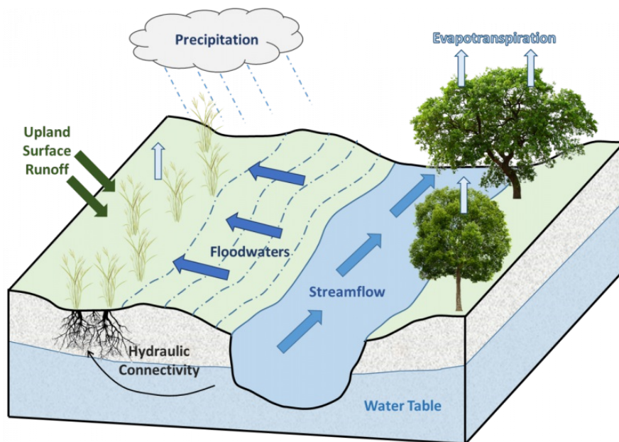
Figure 9. Hydrologic cycling in Floodplain Prairie ecological site.
