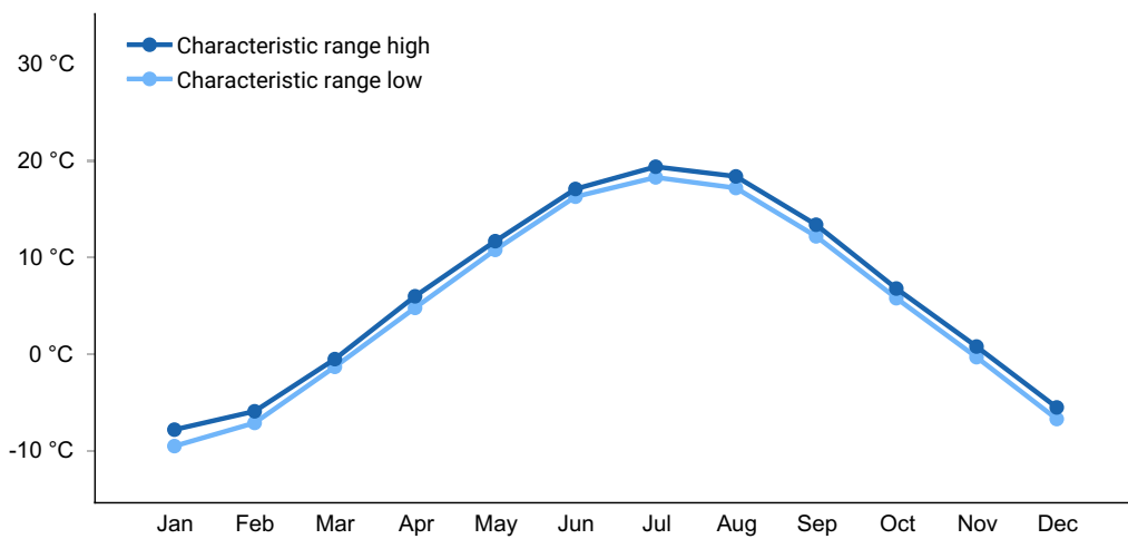
Figure 4. Monthly minimum temperature range
