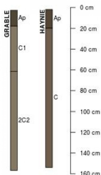
Figure 11. Figure 6. Profile sketches of soil series associated with Sandy/Loamy Floodplain Forest.
