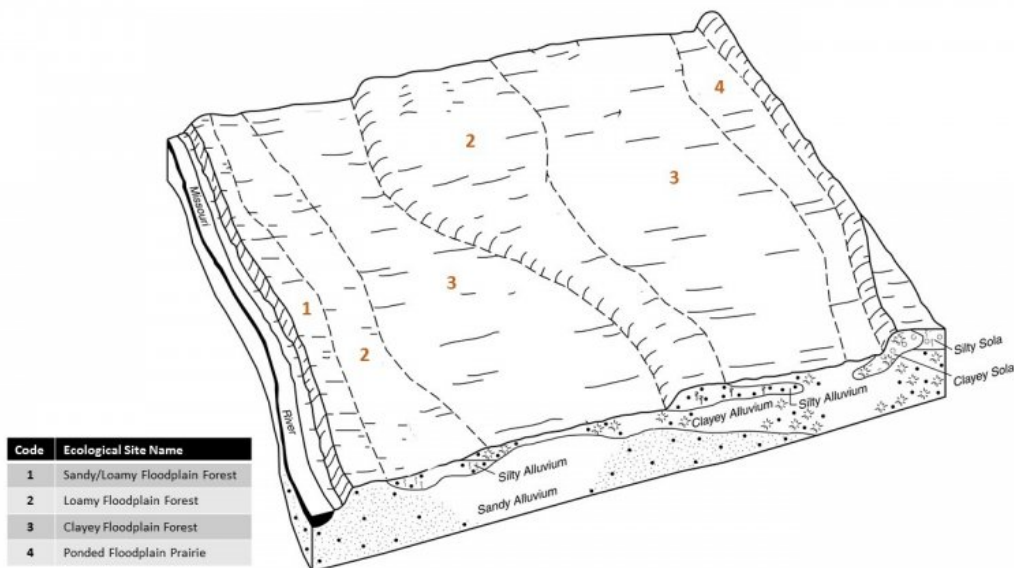
Figure 3. Figure 2. Representative block diagram of Sandy/Loamy Floodplain Forest and associated ecological sites.
