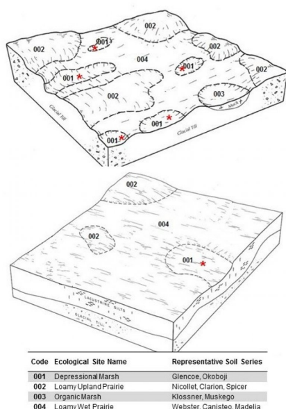
Figure 1. Block diagrams of the representative Depressional Marsh and
