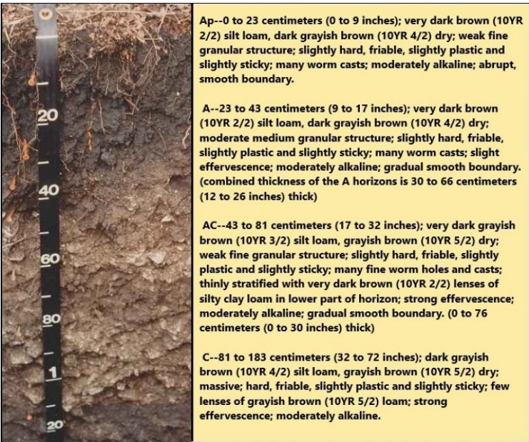
Figure 10. MLRA 76 Ivan soil series profile and description.
