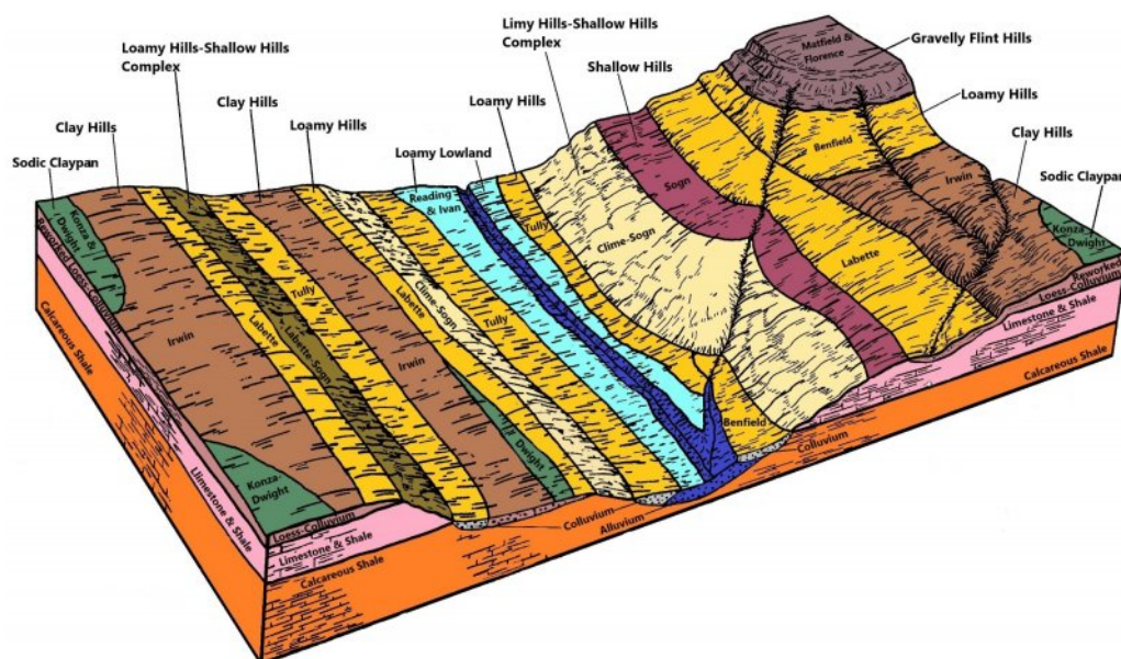
Figure 1. MLRA 76 ESD block diagram.
