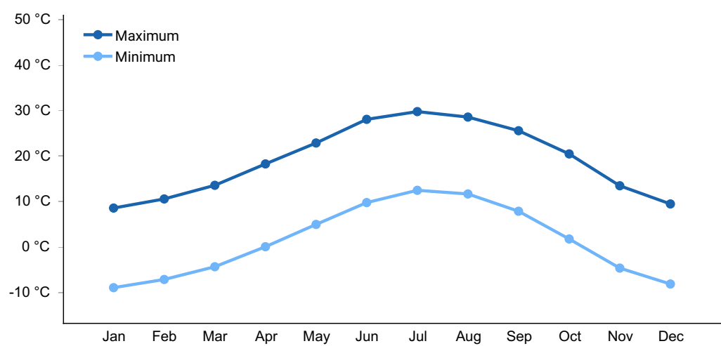
Figure 3. Monthly average minimum and maximum temperature
