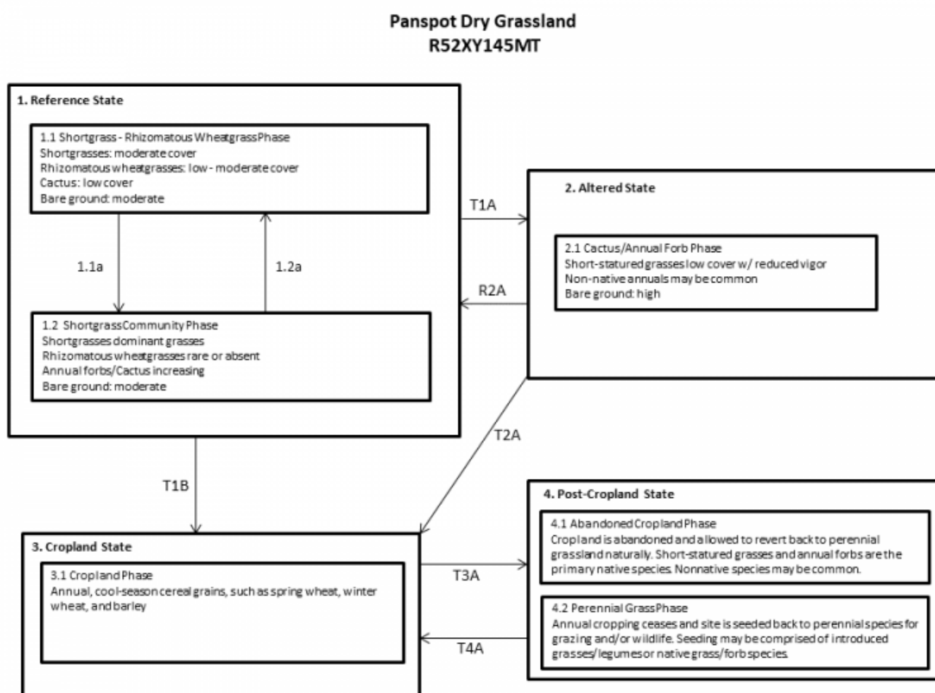
Figure 2. State-and-transition diagram
