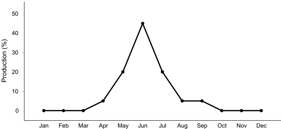
Figure 4. Plant community growth curve (percent production by month). WY1001, 15-19SE upland sites.
